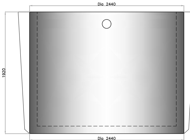
ELEVATION OF TANK
