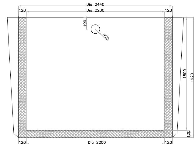
SECTION OF TANK AND LID
