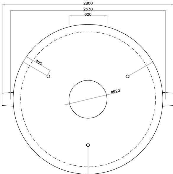
PLAN OF TANK AND BISCUIT LID
