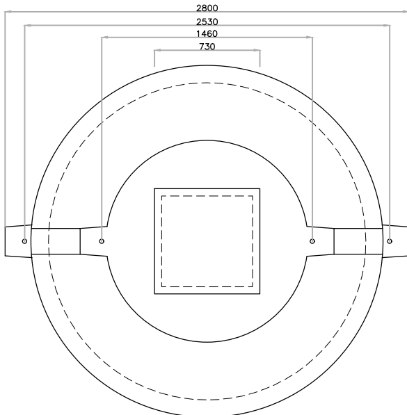
PLAN OF TANK AND DOME LID
