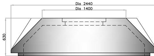
ELEVATION OF DOME LID
