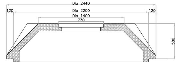
SECTION OF DOME LID
