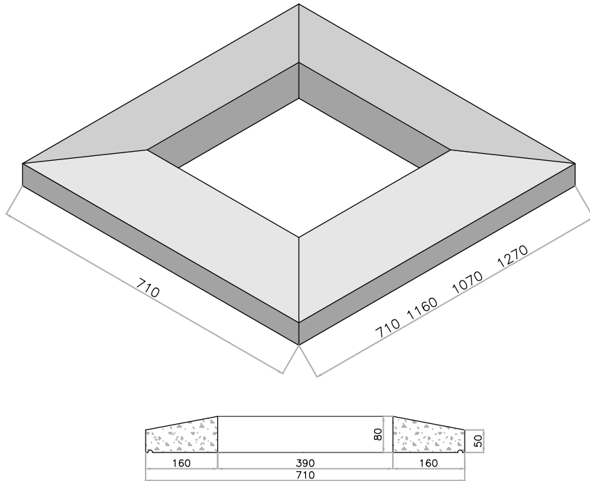
STANDARD CHIMNEY CAP
