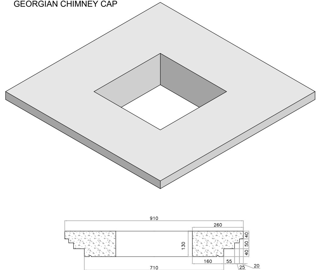
GEORGIAN CHIMNEY CAP
